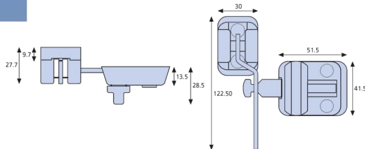
Ventilation Lock
